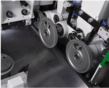
Setting range of the feed rollers opposite left spindle, axial 35 mm
